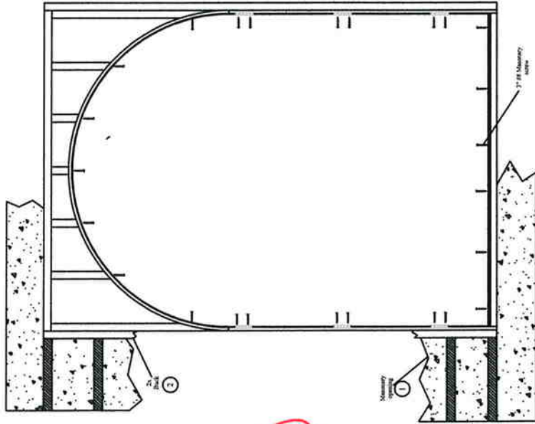
ANCHORING LAYOUT
